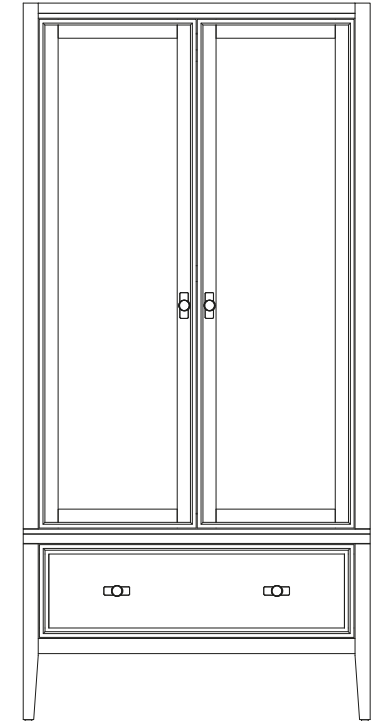
1 DRAWER WARDROBE H: 1900 W: 920 D: 580
