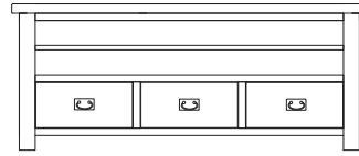
LARGE TV UNIT WITH DRAWERS H: 600 W: 1450 D: 425
