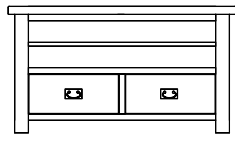
TV UNIT WITH DRAWERS H: 600 W: 1080 D: 425
