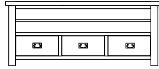
LARGE TV UNIT WITH DRAWERS H: 656 W: 1450 D: 425
